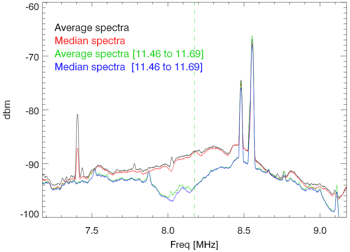
01aug18 average spectra. hf 8Mhz dipole 1. RBW=10KHz
