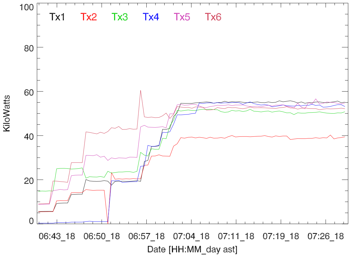
TxPwr by Tx. 18mar17:H3156. Paul Bernhardt
