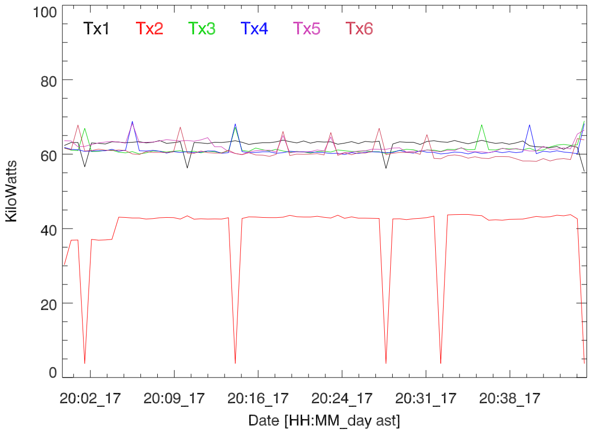
TxPwr by Tx. 17mar17:H3156. Paul Bernhardt
