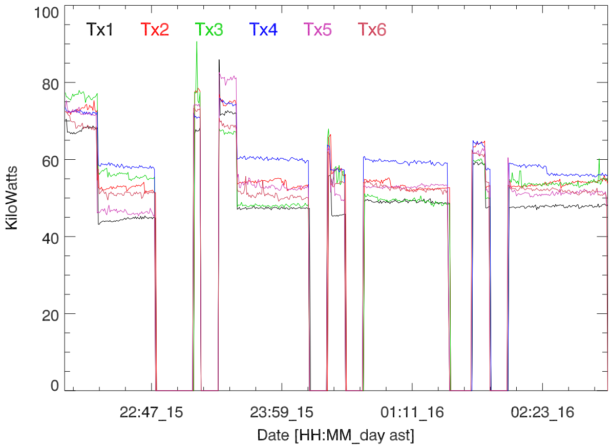
TxPwr by Tx. 15mar17:T2604. Min-Chang Lee
