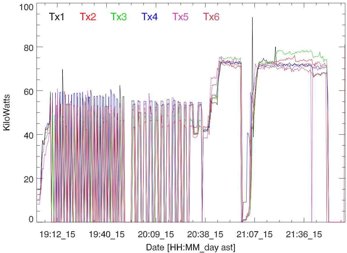
TxPwr by Tx. 15mar17:H3156. Paul Bernhardt
