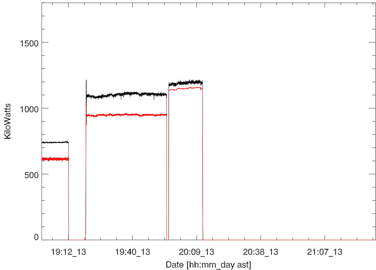
GD 430 Transmitted power for: 13mar17:T3156. Paul Bernhardt
