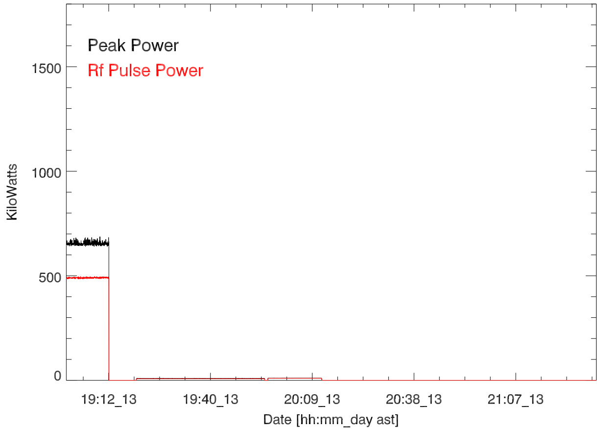
CH 430 Transmitted power for: 13mar17:T3156. Paul Bernhardt
