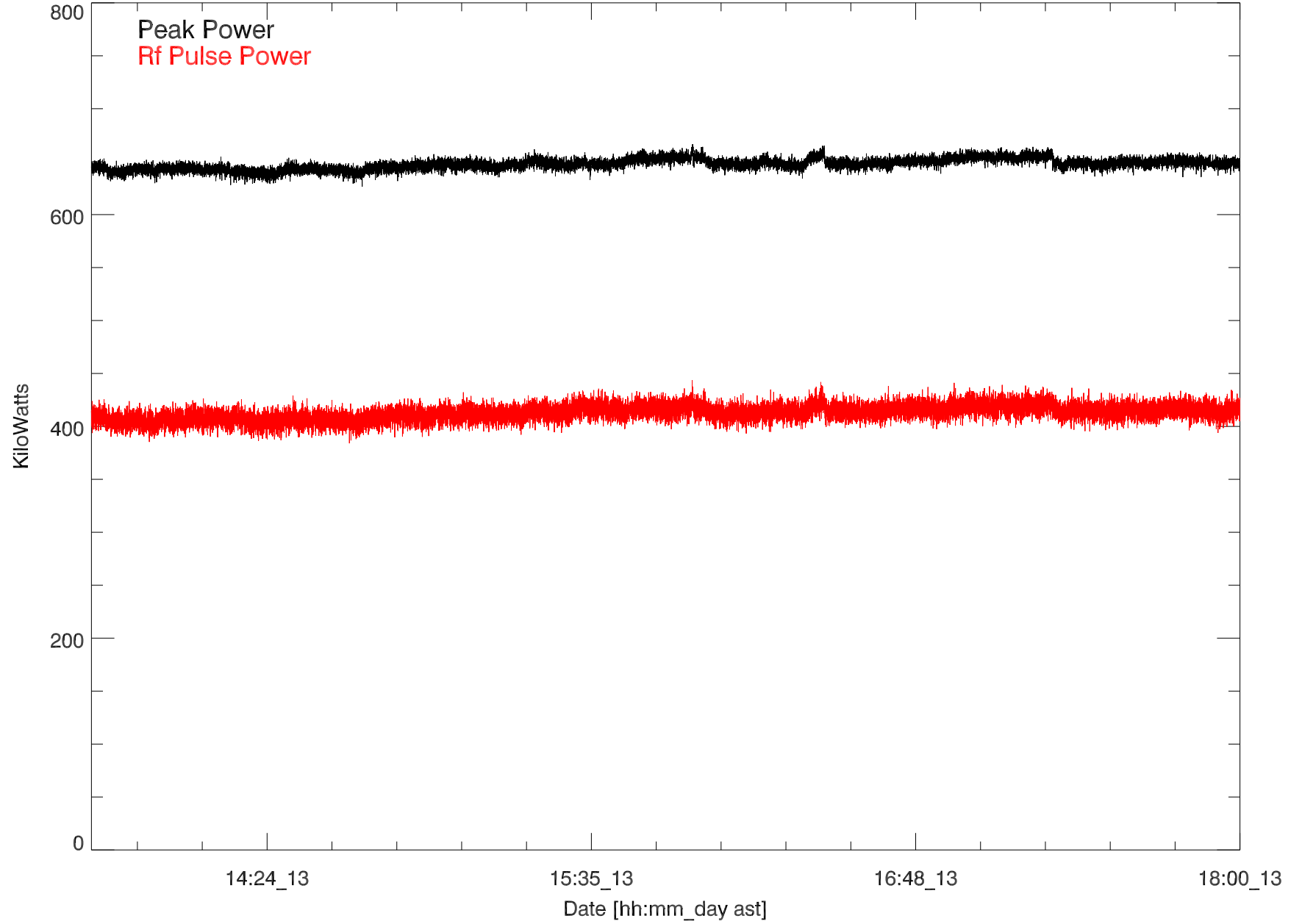
GD 430 Transmitted power for: 13jun19:H3368 edlyn exp13.06
