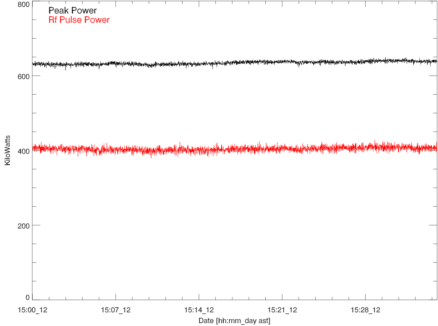
GD 430 Transmitted power for: 12jun19:H3337 paul exp12.08
