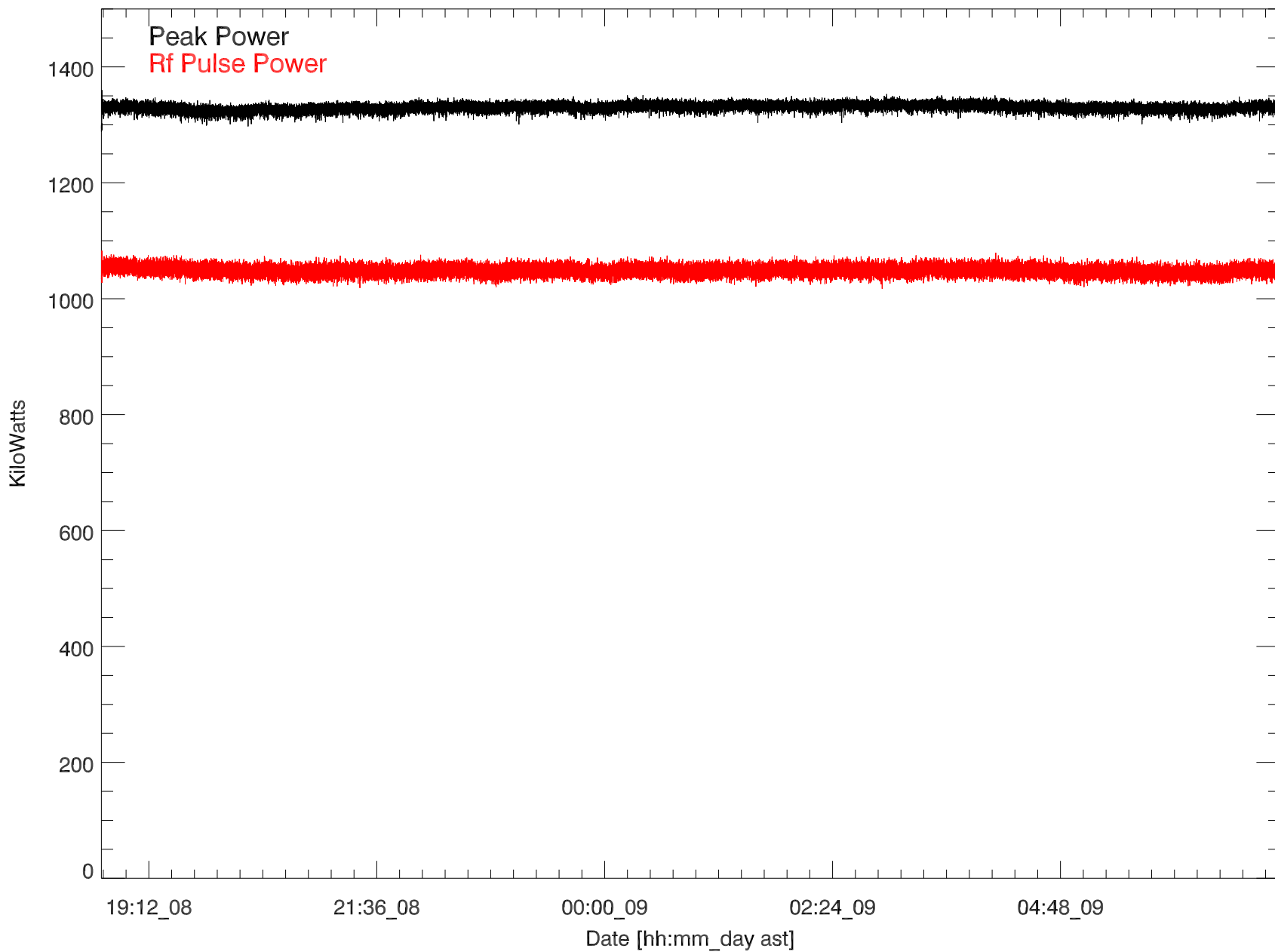
GD 430 Transmitted power for: 08nov18:T2374 (no hf)
