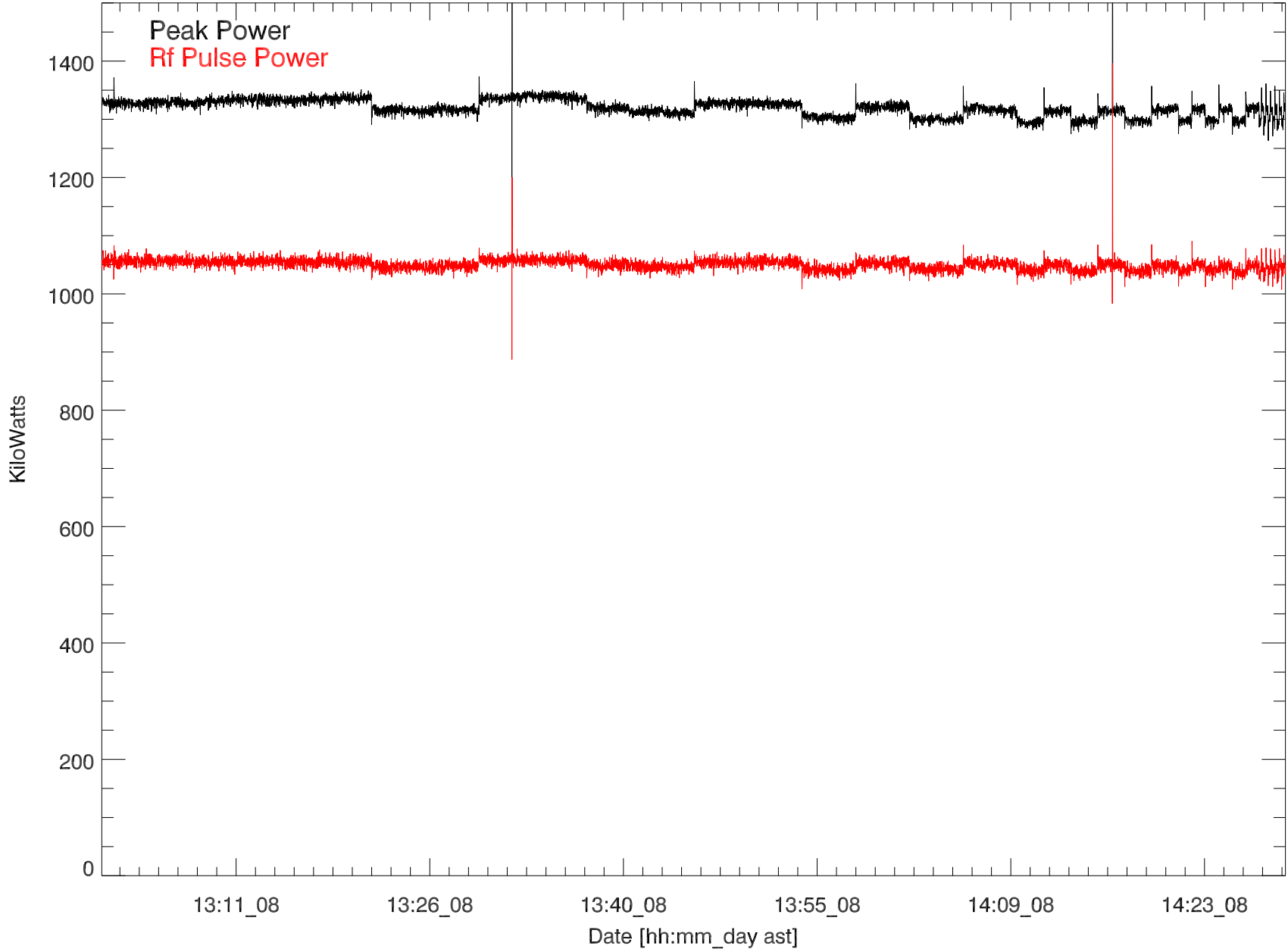
GD 430 Transmitted power for: 08nov18:H3211
