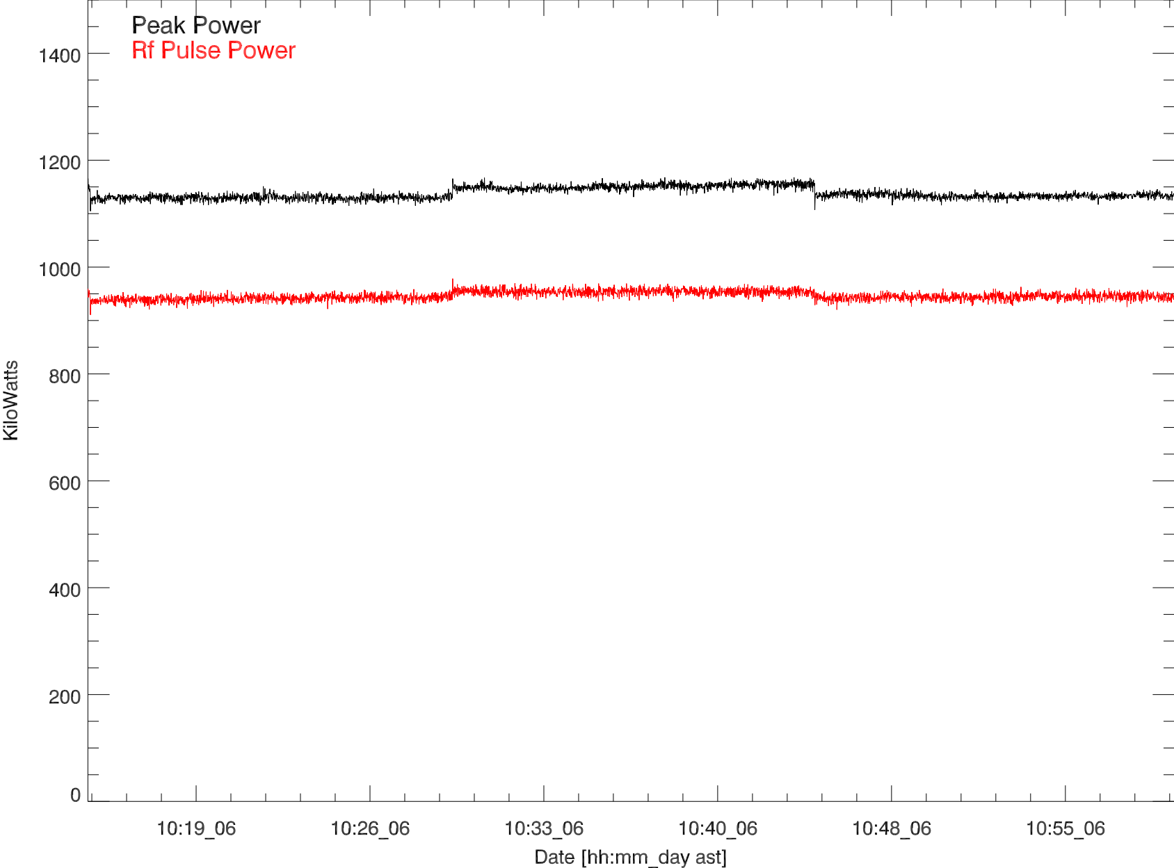
GD 430 Transmitted power for: 06nov18:H3252
