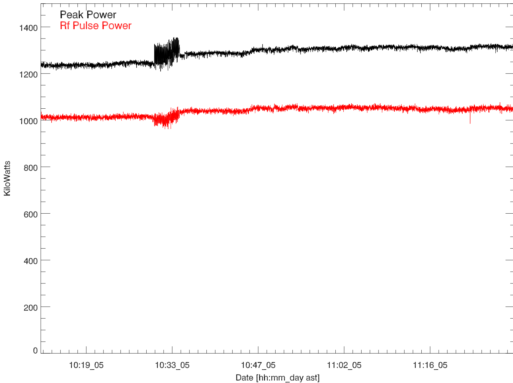
GD 430 Transmitted power for: 05nov18:H3252
