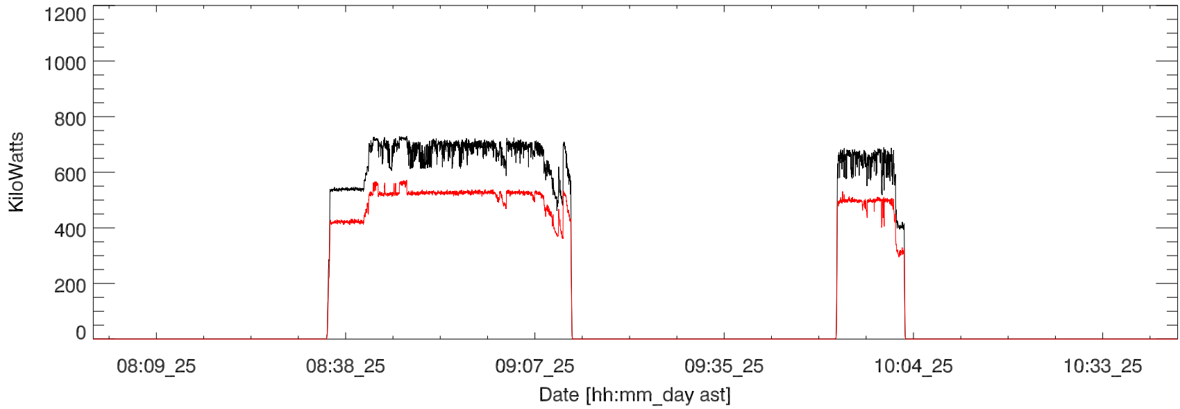
GD 430 Transmitted power for: 25jul17:H3206. Chris Fallen
