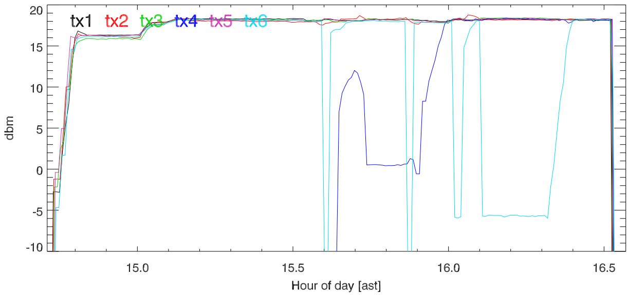
170201 8 Mhz Band tx power. rf coupler output. . 8 MHz test
