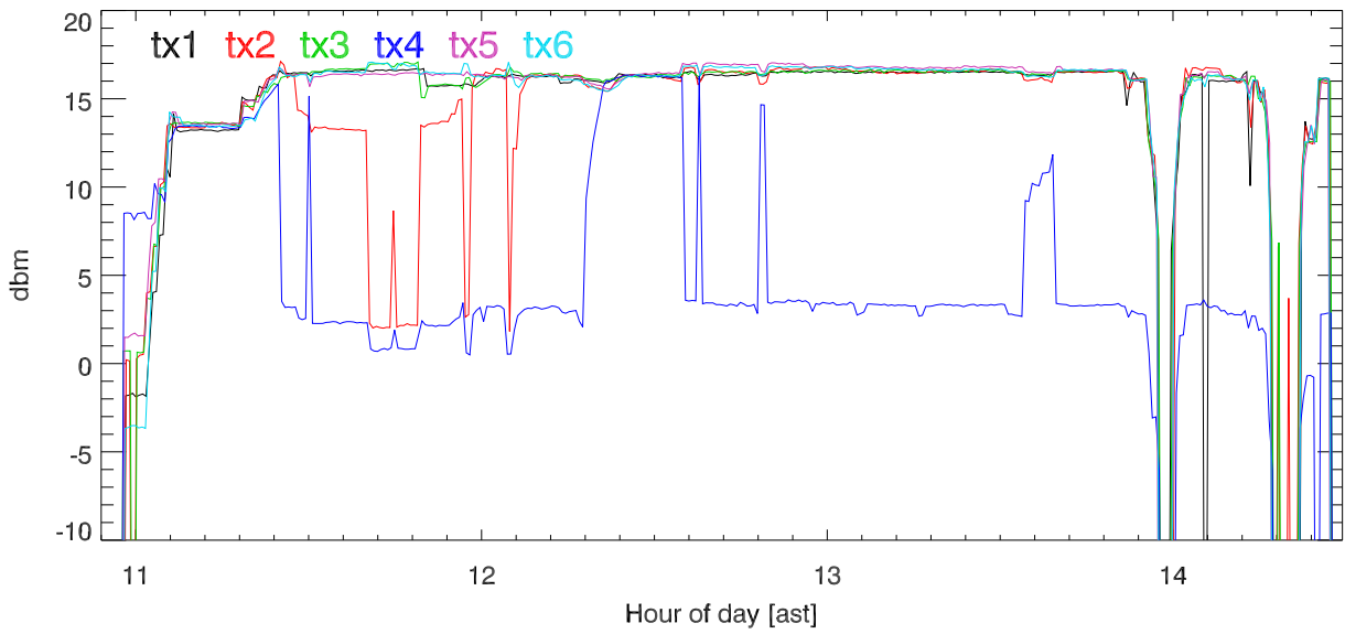
170201 5 MHz Band tx power. rf coupler output. . 5Mhz test.
