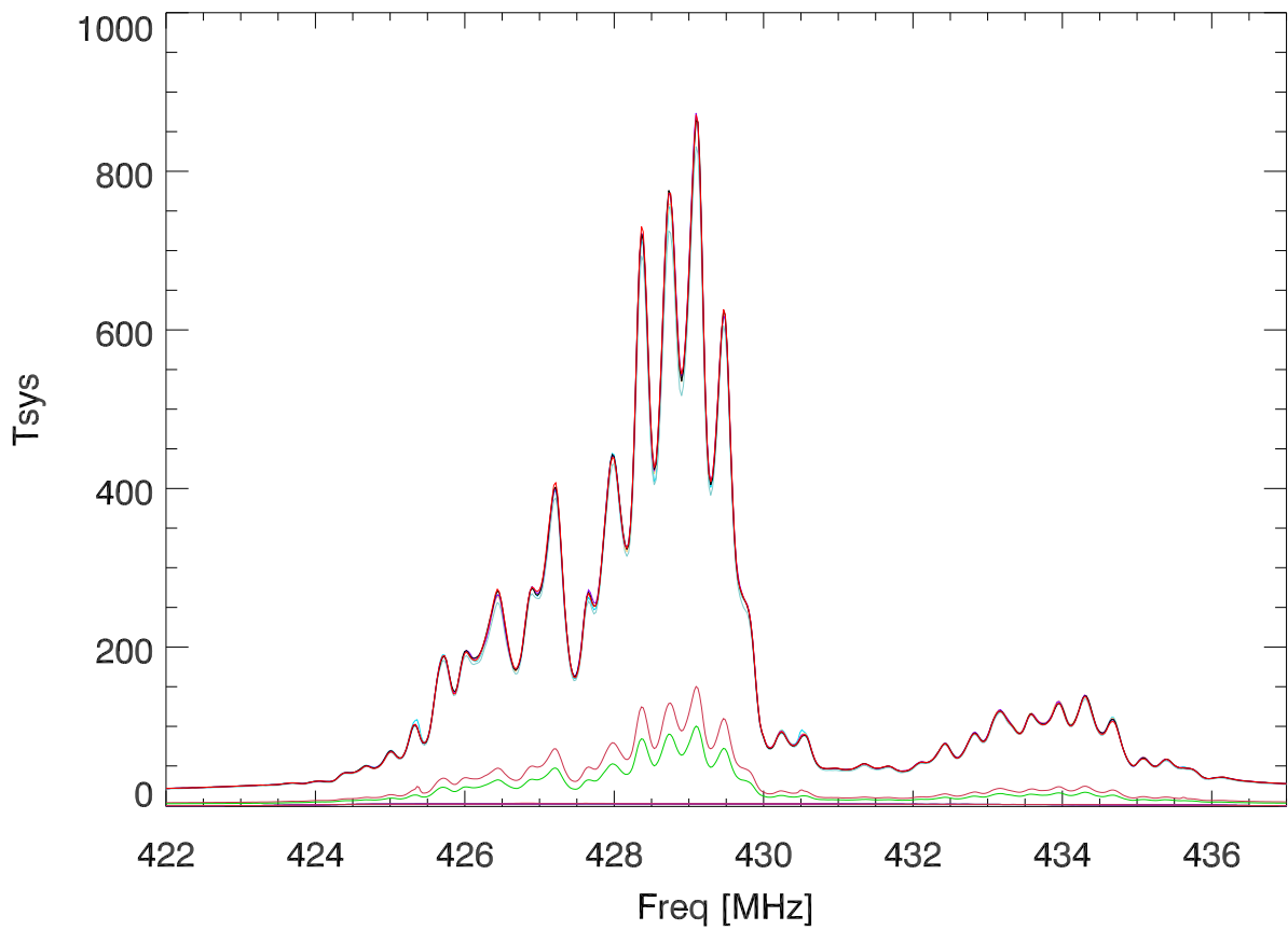
26jan17 hf test. 430 spectra with tx Arcing
