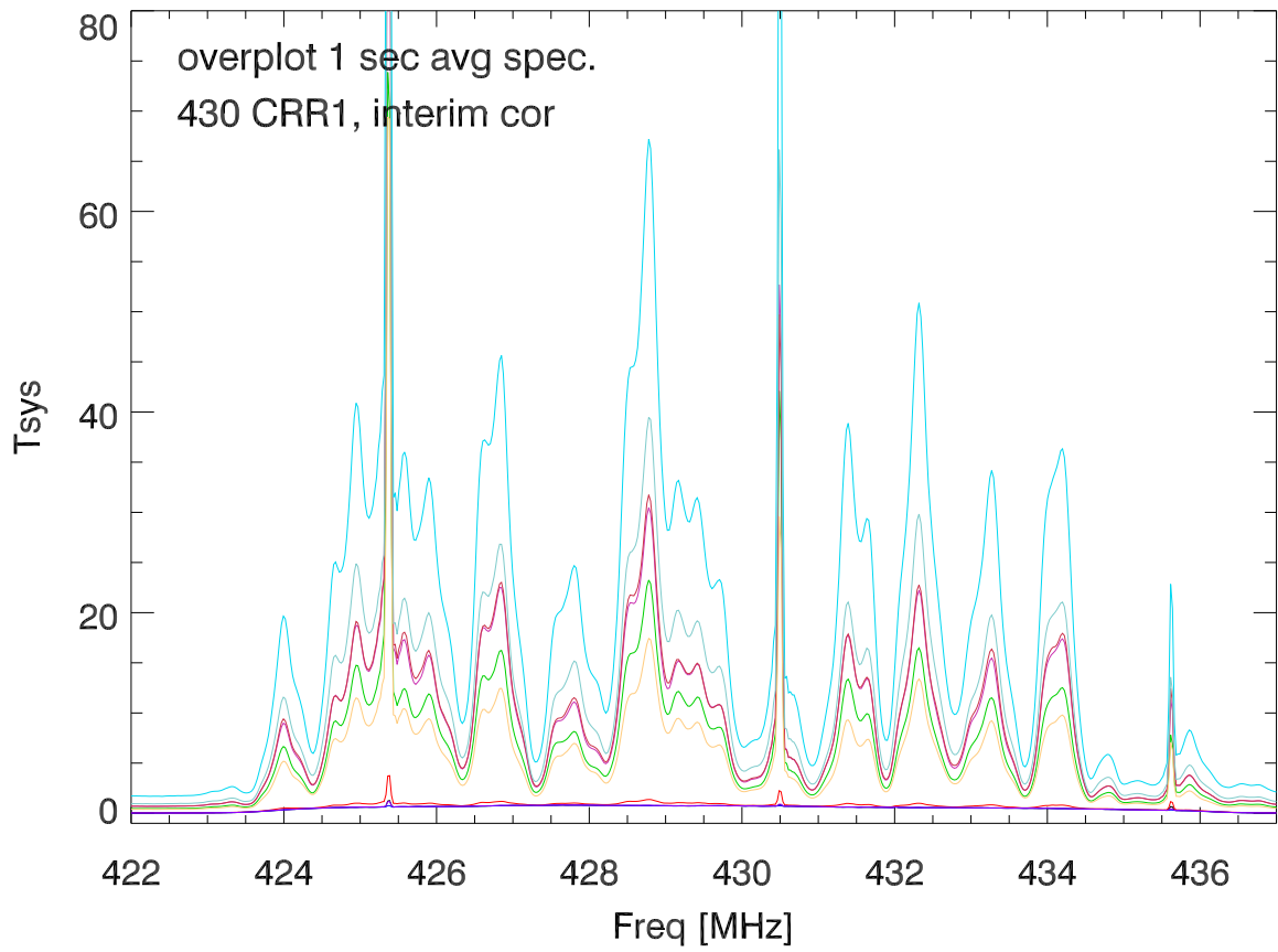
29oct15 hf test. 430 spectra with external arcing
