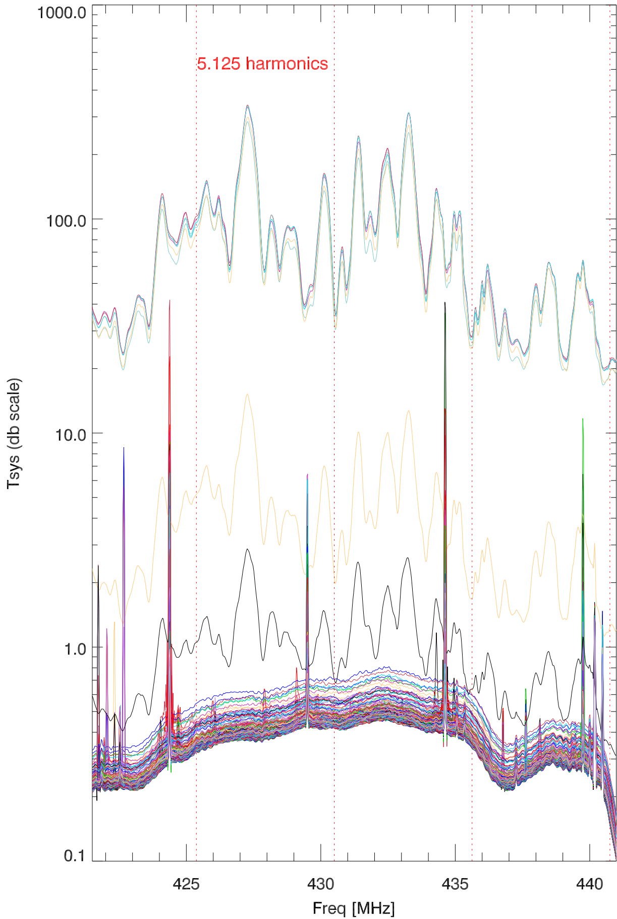
31may16 overplot ch spectra hours: 11.8 to 12.2
