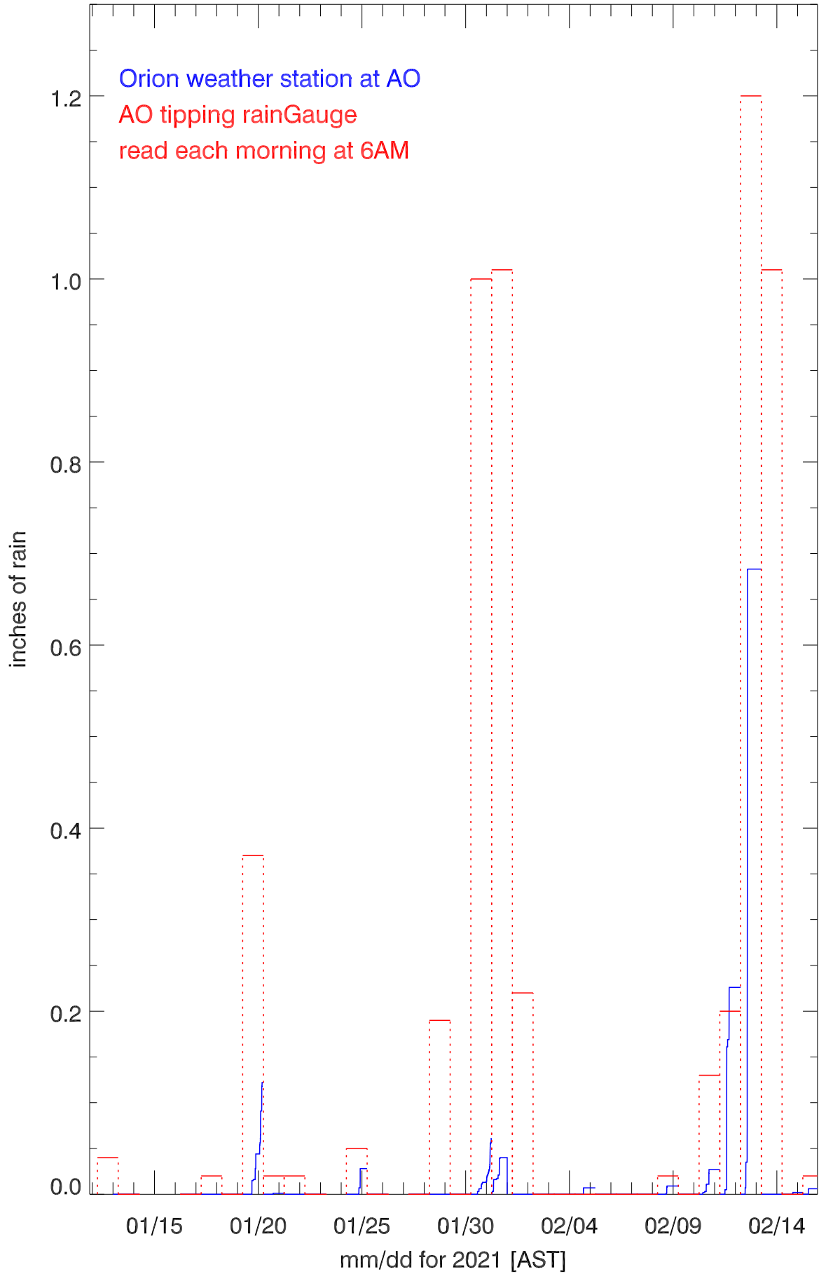
Compare orion rain gauge with AO tipping rain gage
