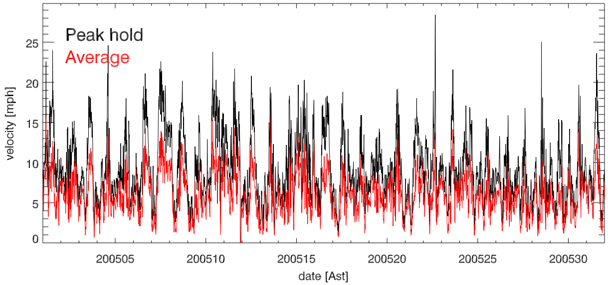
may20 Avg & Peak velocities vs date (over 15.0 minutes)
