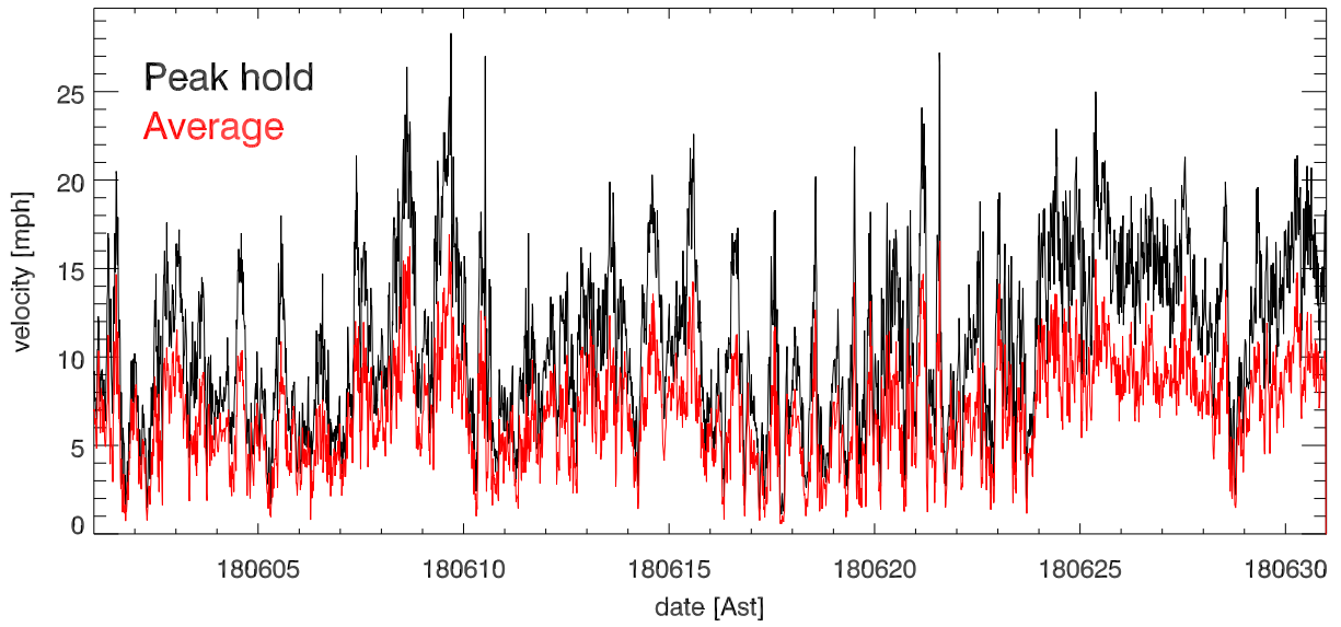
jun18 Avg & Peak velocities vs date (over 15.0 minutes)
