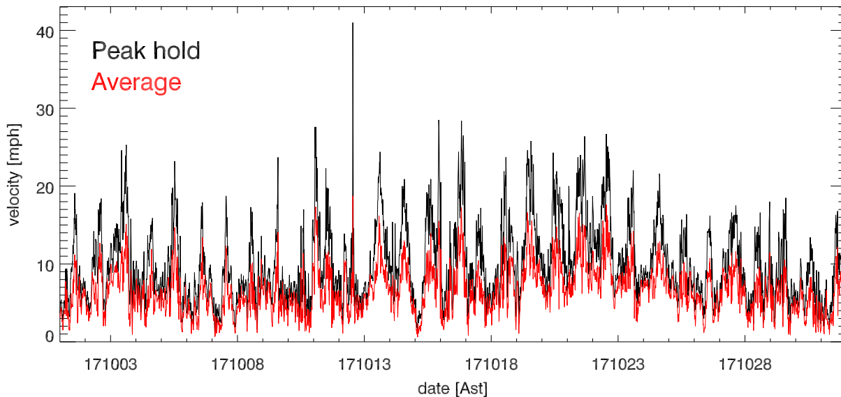
oct17 Avg & Peak velocities vs date (over 15.0 minutes)
