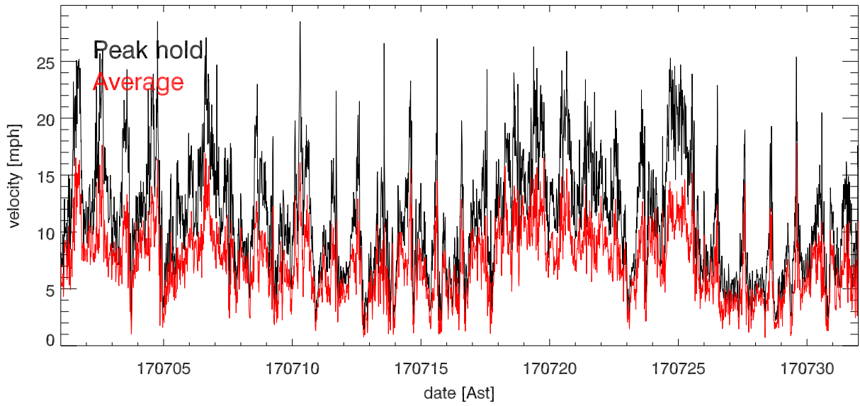
Jul17 Avg & Peak velocities vs date (over 15.0 minutes)
