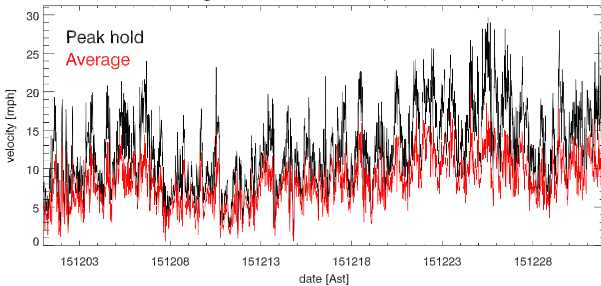
dec15 Avg & Peak velocities vs date (over 15.0 minutes)
