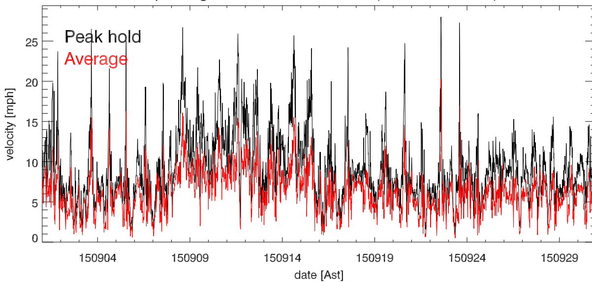
sep15 Avg & Peak velocities vs date (over 15.0 minutes)
