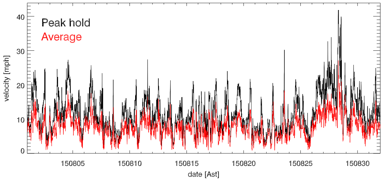
aug15 Avg & Peak velocities vs date (over 15.0 minutes)
