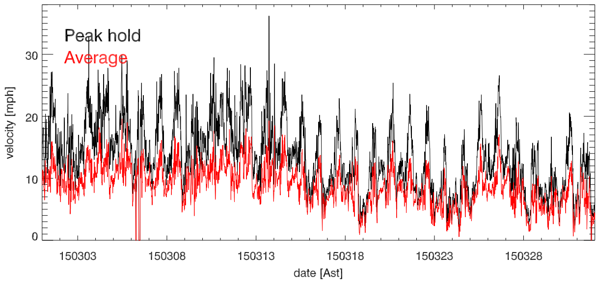
mar15 Avg & Peak velocities vs date (over 15.0 minutes)
