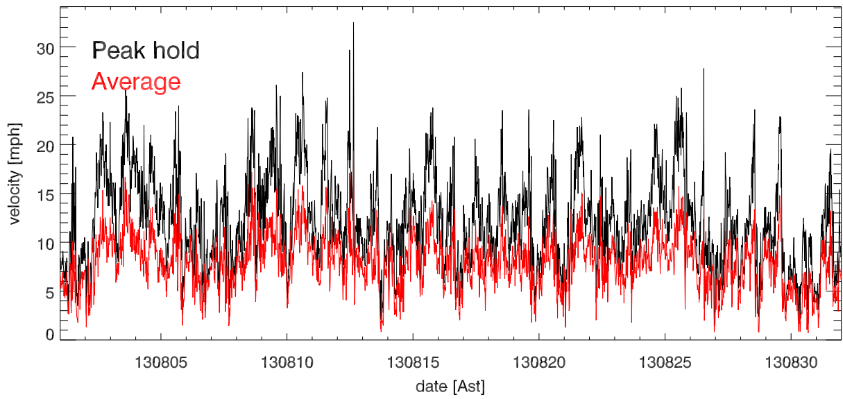
aug13 Avg & Peak velocities vs date (over 15.0 minutes)
