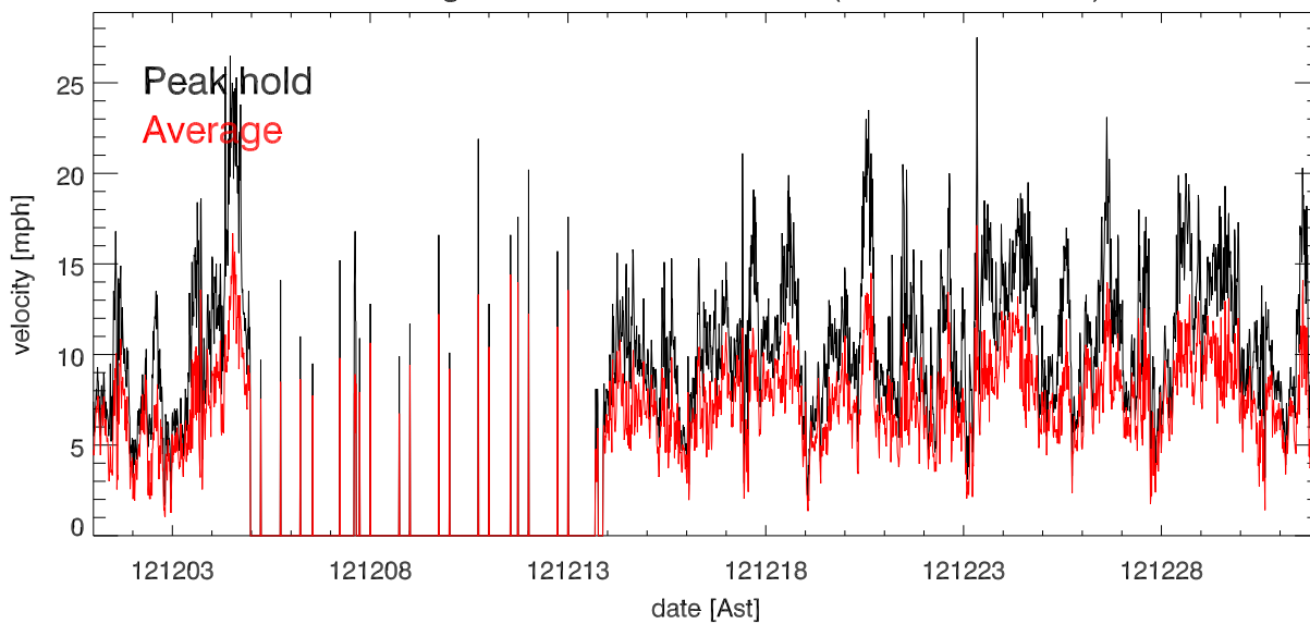
dec12 Avg & Peak velocities vs date (over 15.0 minutes)
