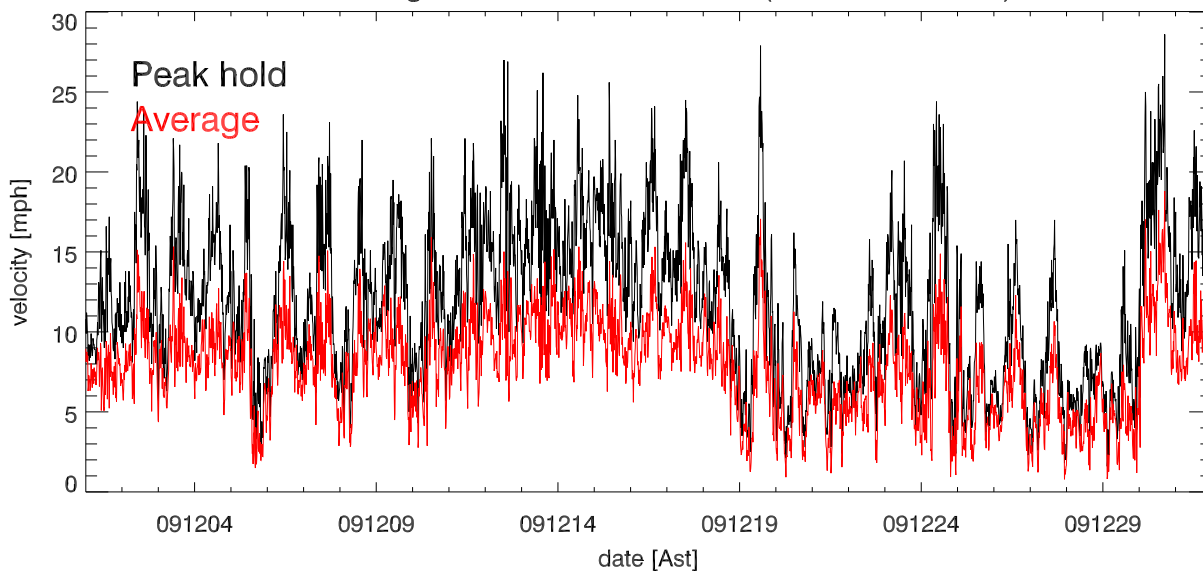
dec09 Avg & Peak velocities vs date (over 15.0 minutes)
