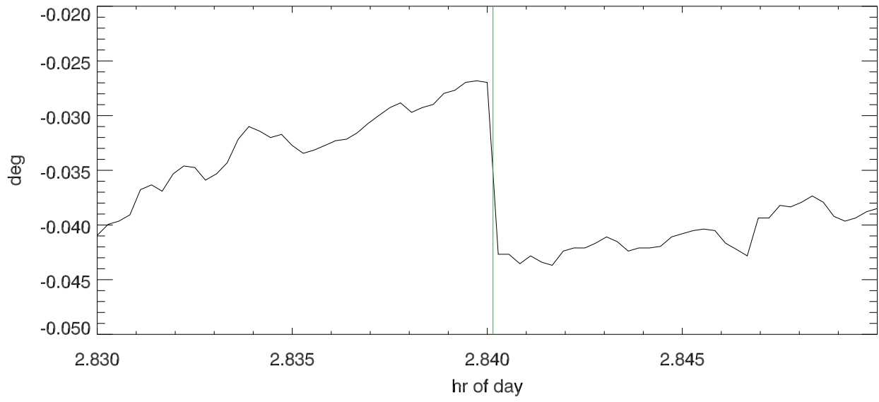
10oct19 az encoder jump. Az encoder Difference vs hr of day
