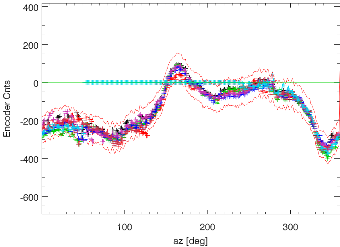
Azimuth encoder difference daily averages. (EncoderCnts).
