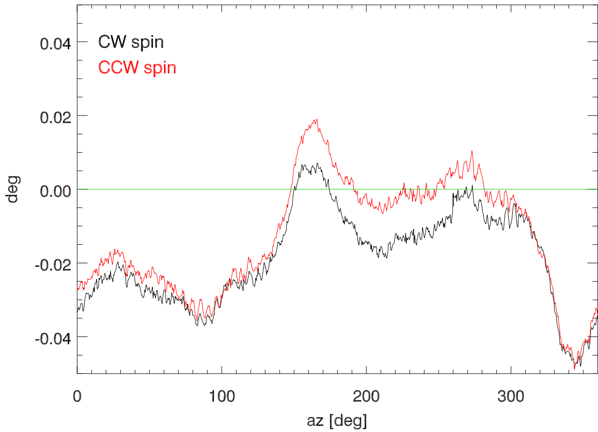
191016 azimuth encoder difference (deg) vs az (after enc1,2 reset)
