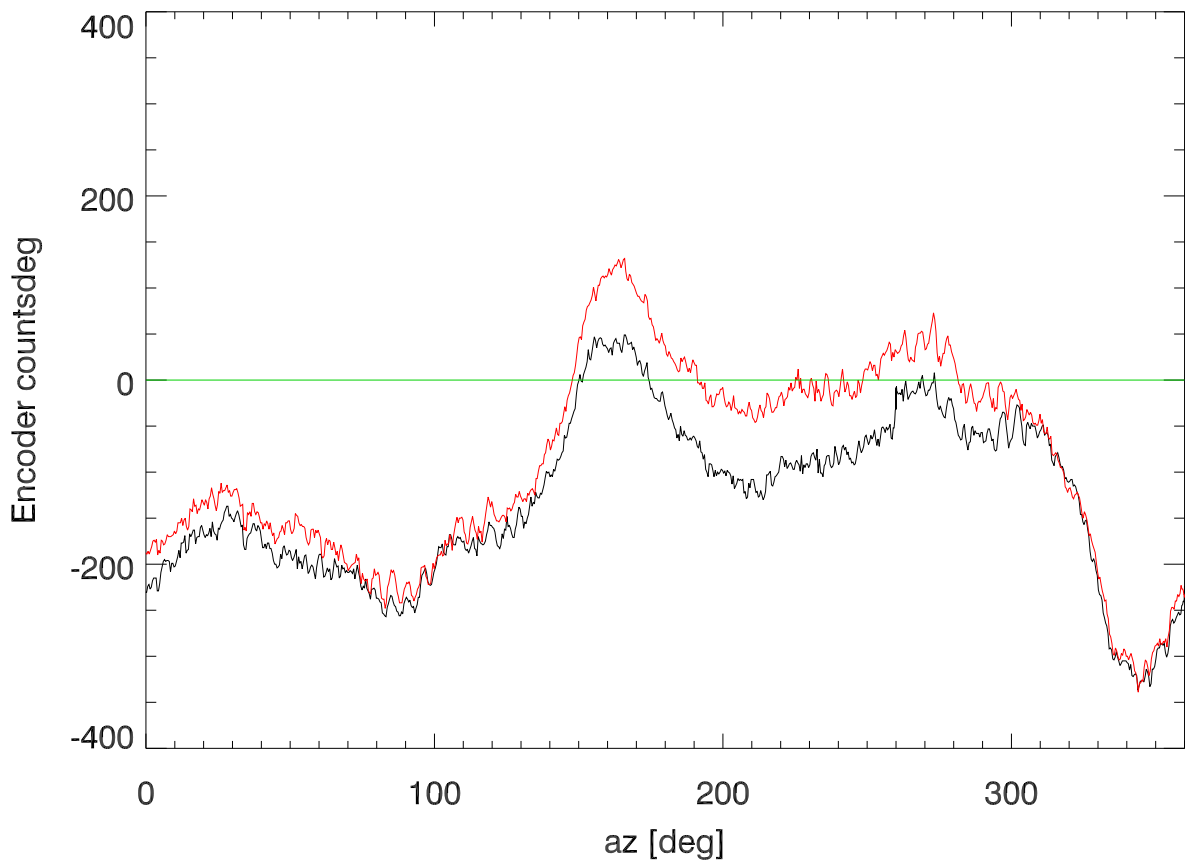
azimuth encoder difference (Encoder Cnts) vs az
