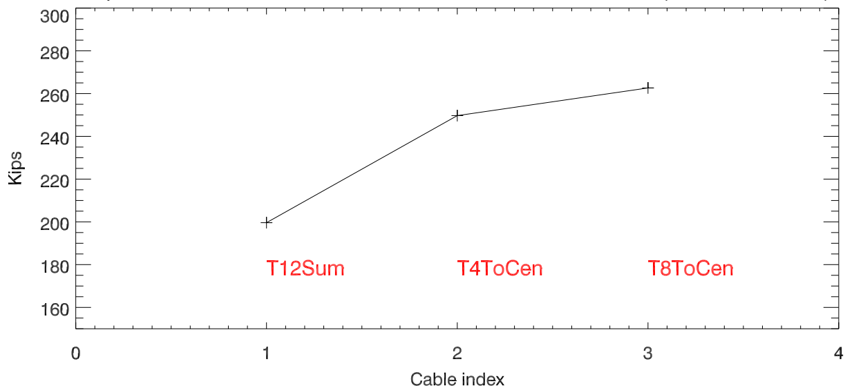
sept2020 catwalk to tower cable horizontal radial tensions (sum T12 cables)
