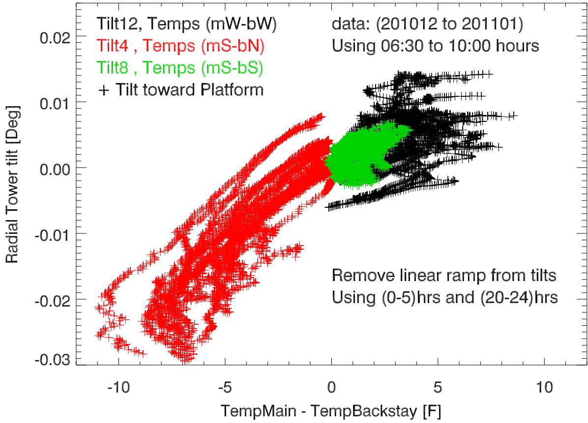
radial tower tilt vs (main-backstay) cable tempDif.
