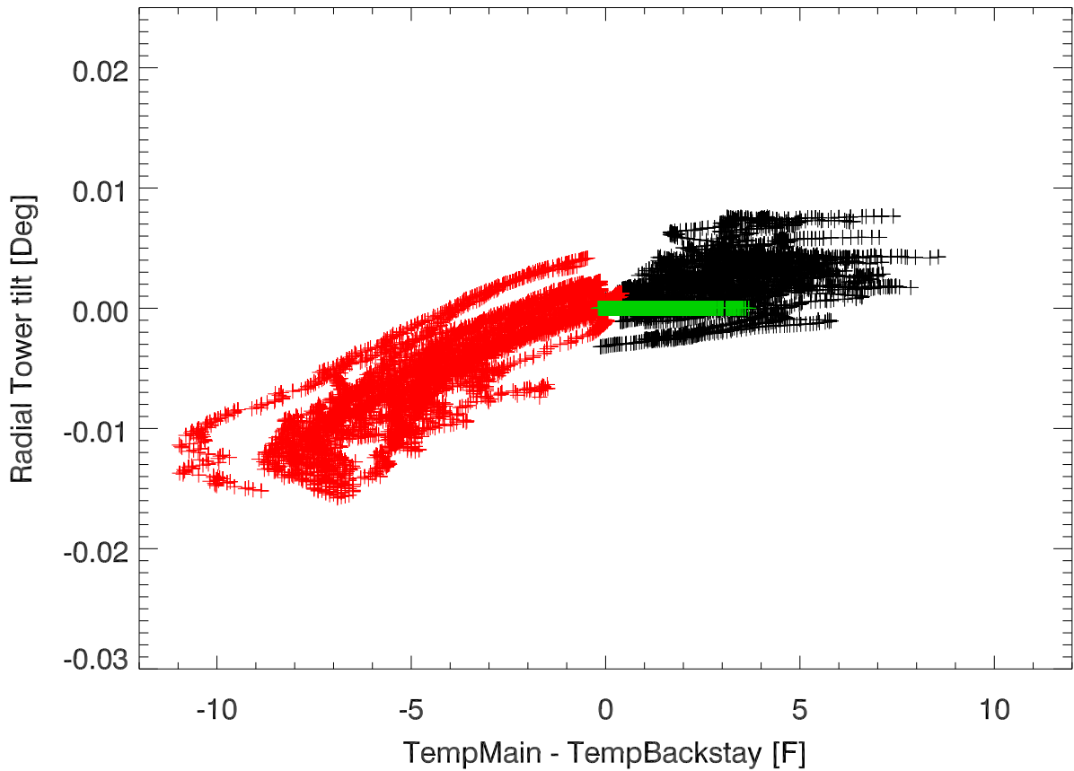
Tangential tower tilt vs (main-backstay) cable tempDif.
