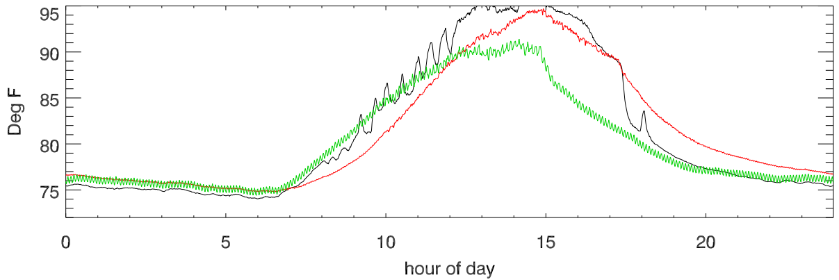
Cable temps vs hour of day. Main Cables for 20201025
