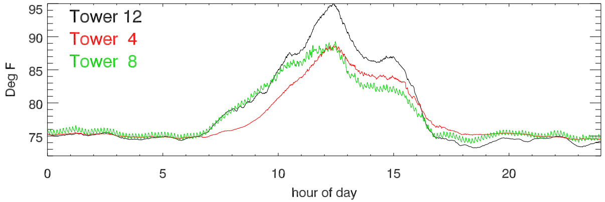
Cable temps vs hour of day. Main Cables for 20201012
