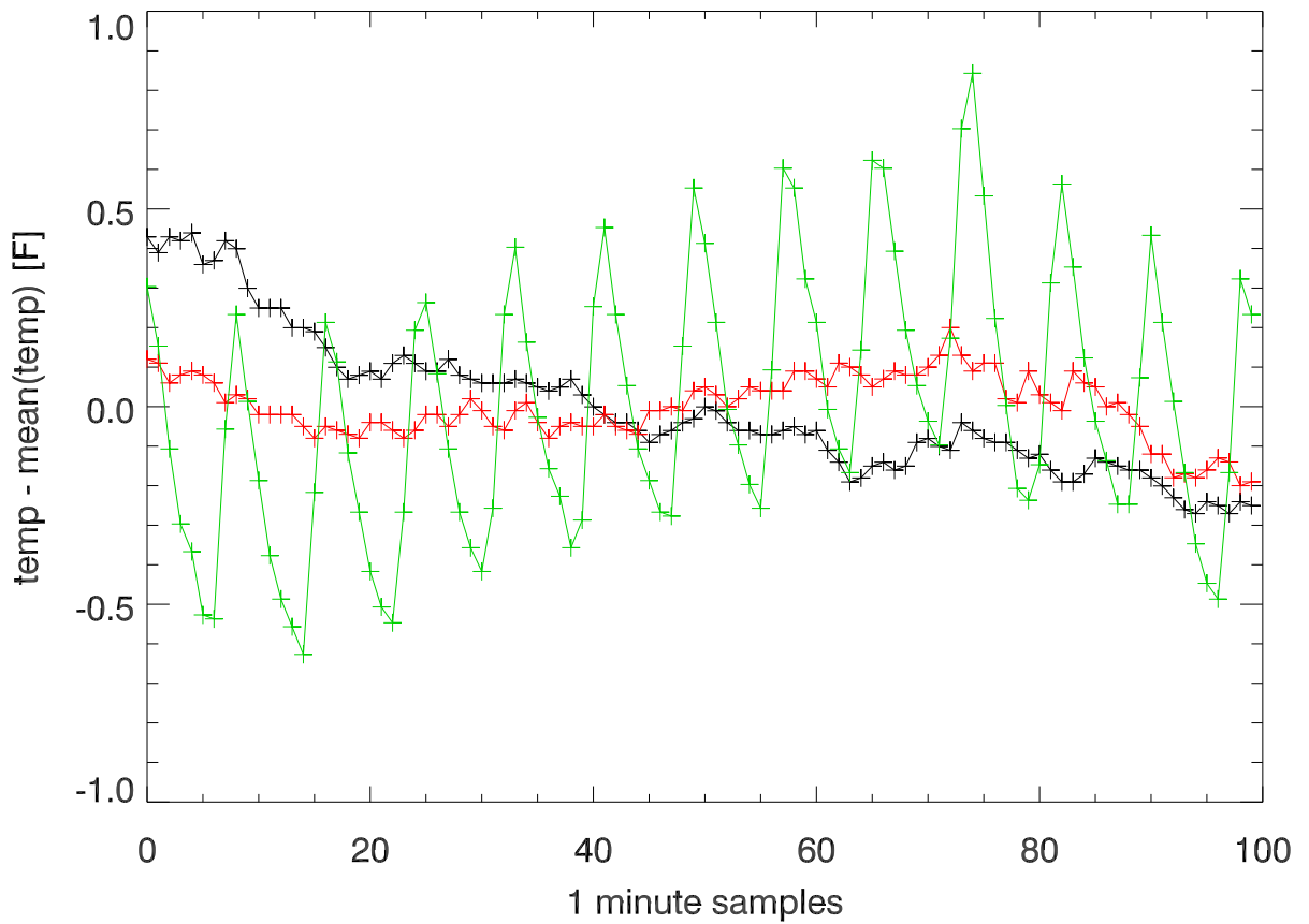
Temp - mean(temp) for 1st 100 minutes(samples). backstayTemps
