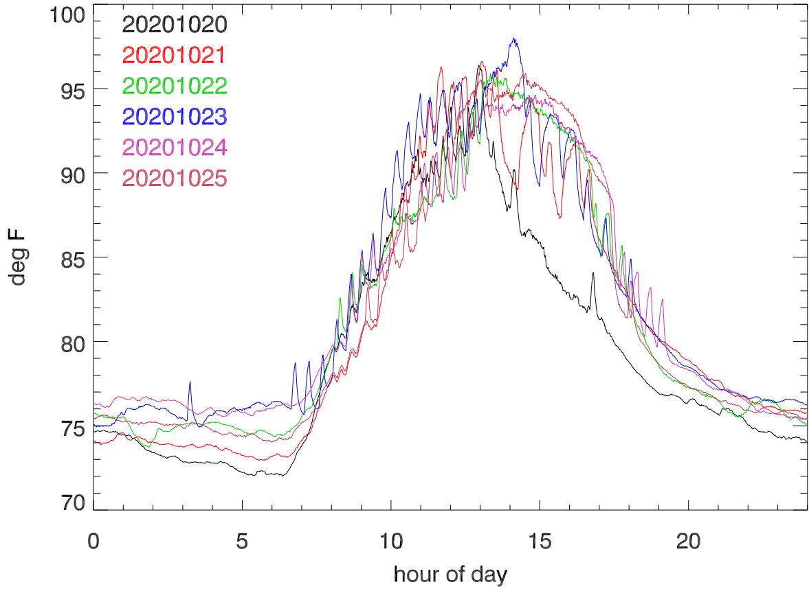
Main cable temps vs hour of day. Tower12
