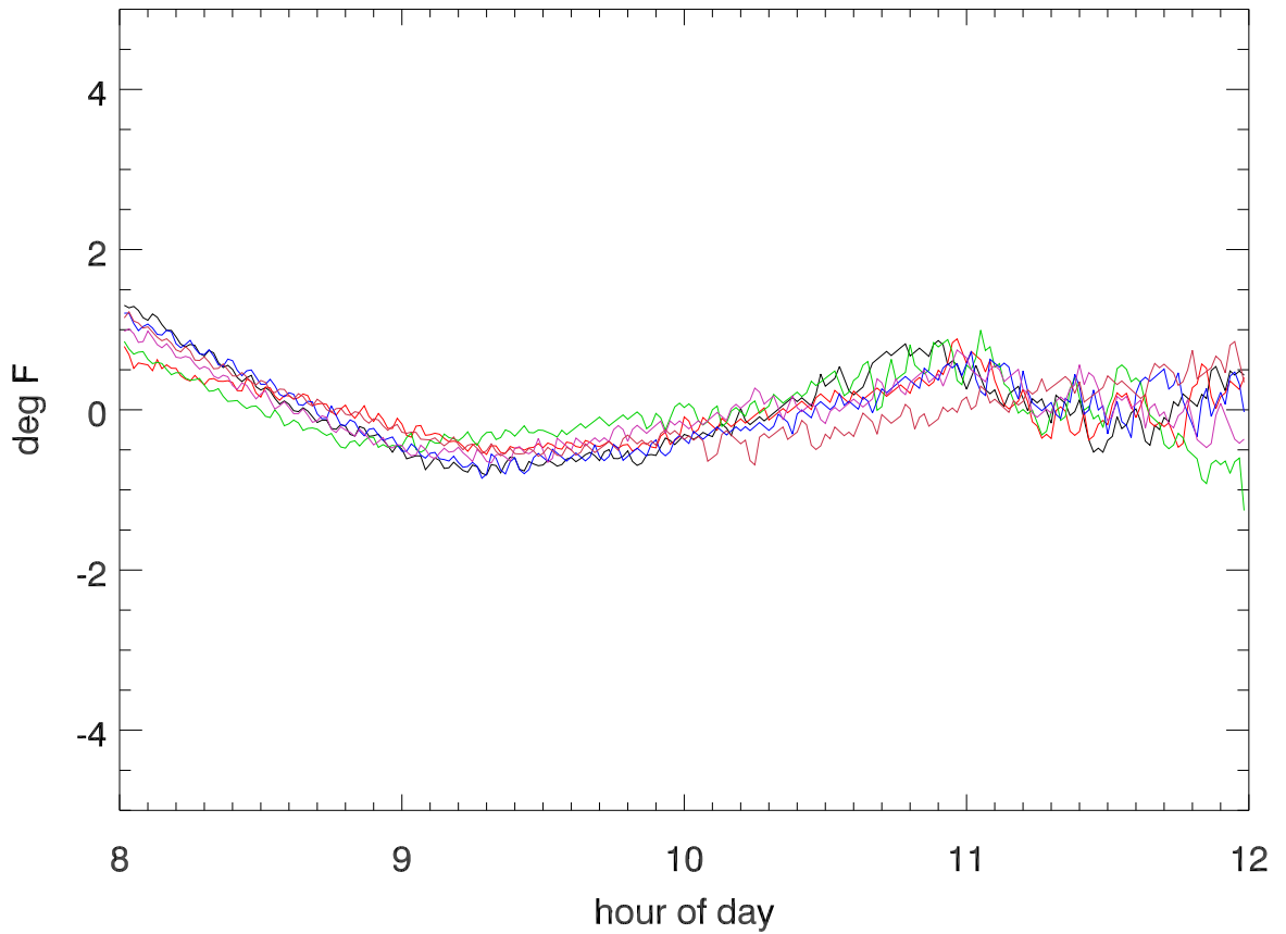
(Main cable temps -linear fit) vs hour of day. Tower4
