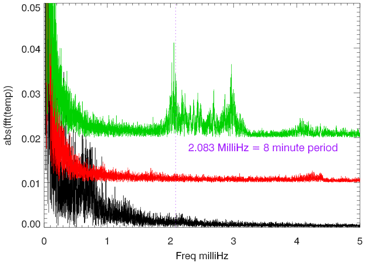
Freq spectrum of temps for 15 days of data. BackstayTemps
