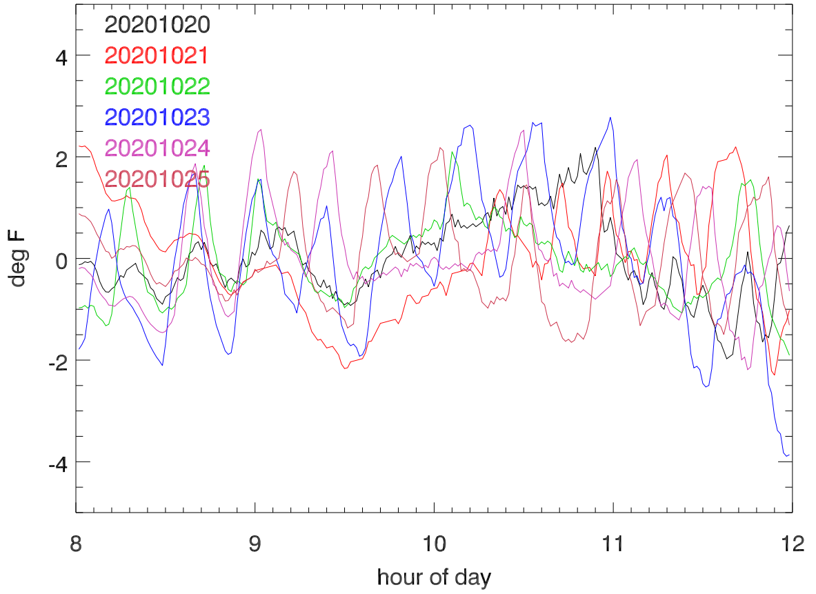
(Main cable temps -linear fit) vs hour of day. Tower12
