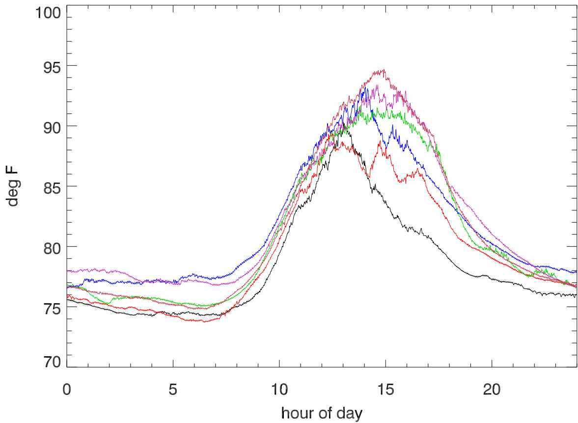
Main cable temps vs hour of day. Tower4
