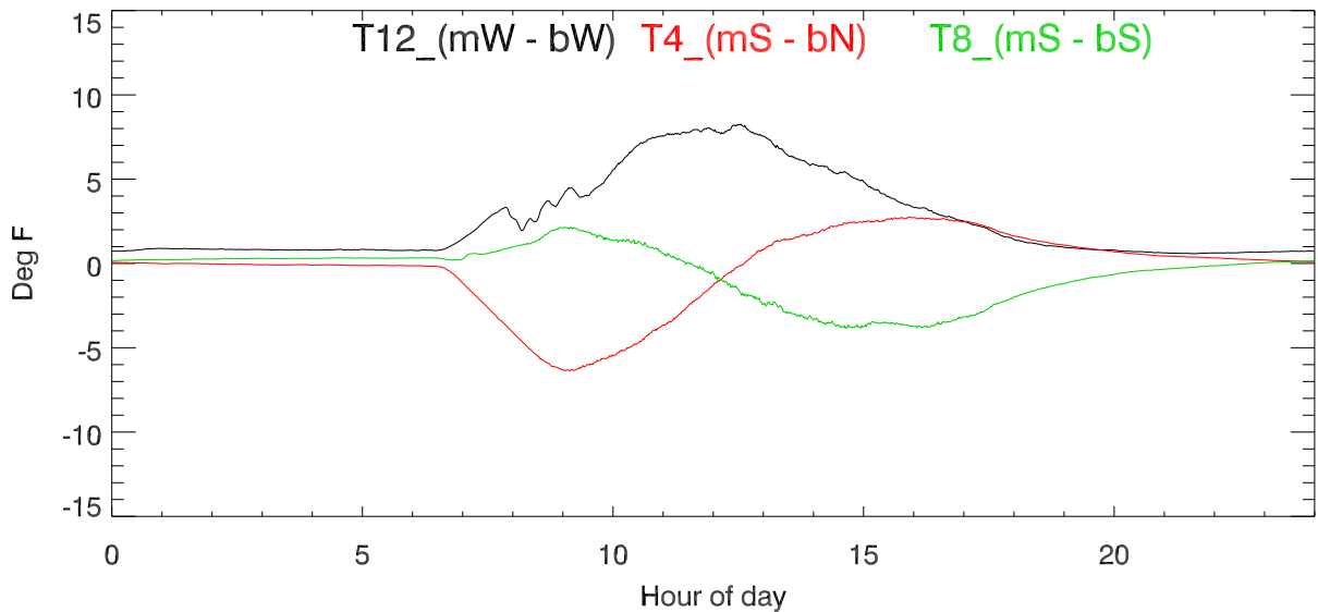
Average aux cable temp difference (main-backstay) vs hour of day.
