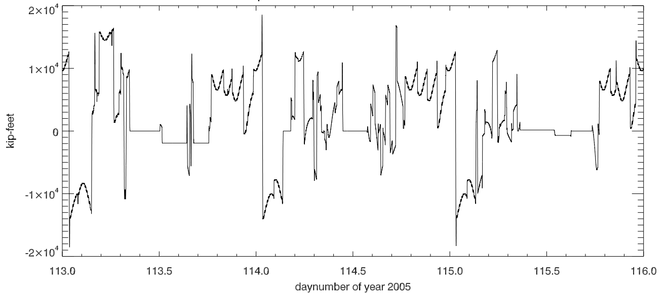
23-25apr05 unbalanced moment at corner 12.
