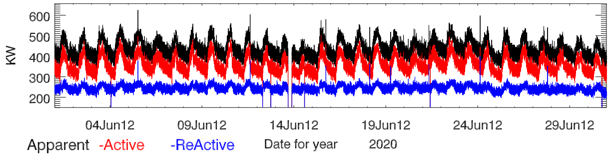
Site power data for jun2020. Power
