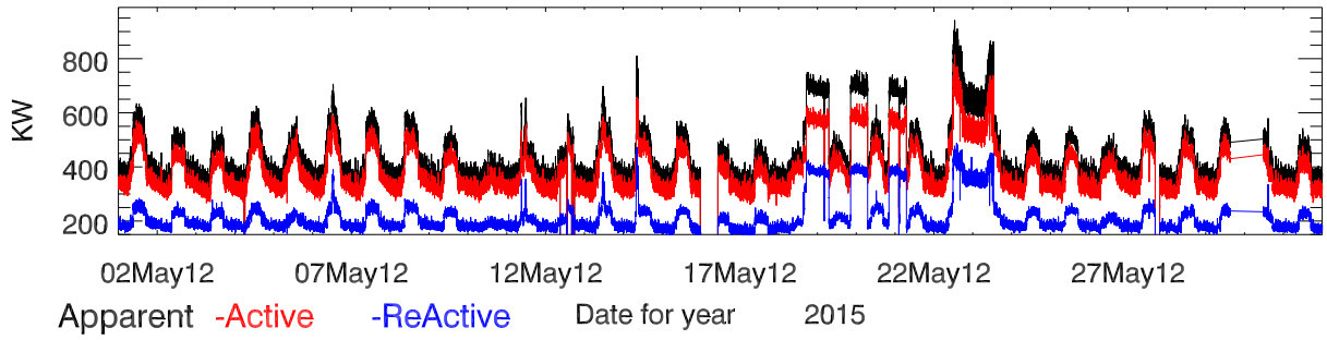
Site power data for may2015. Power
