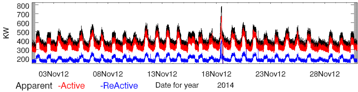
Site power data for nov2014. Power
