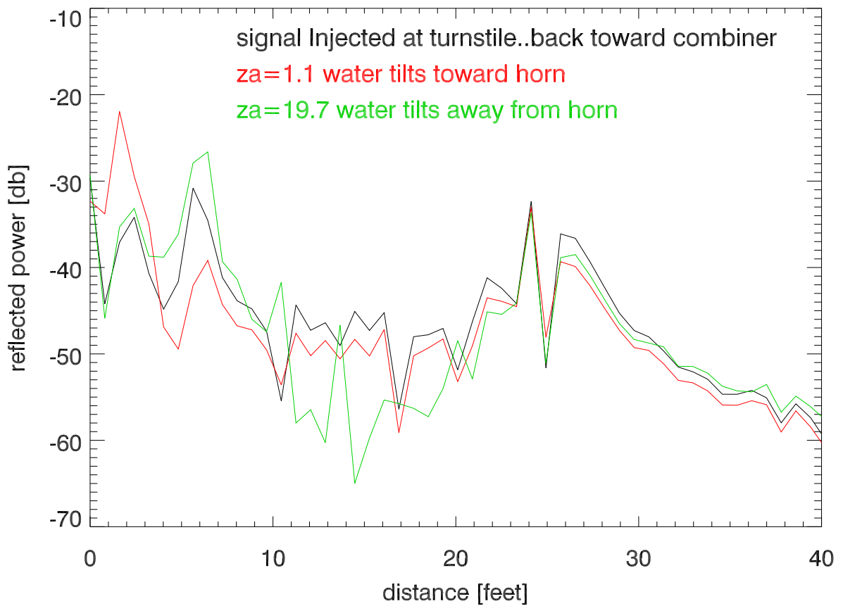
reflected power vs distance.
