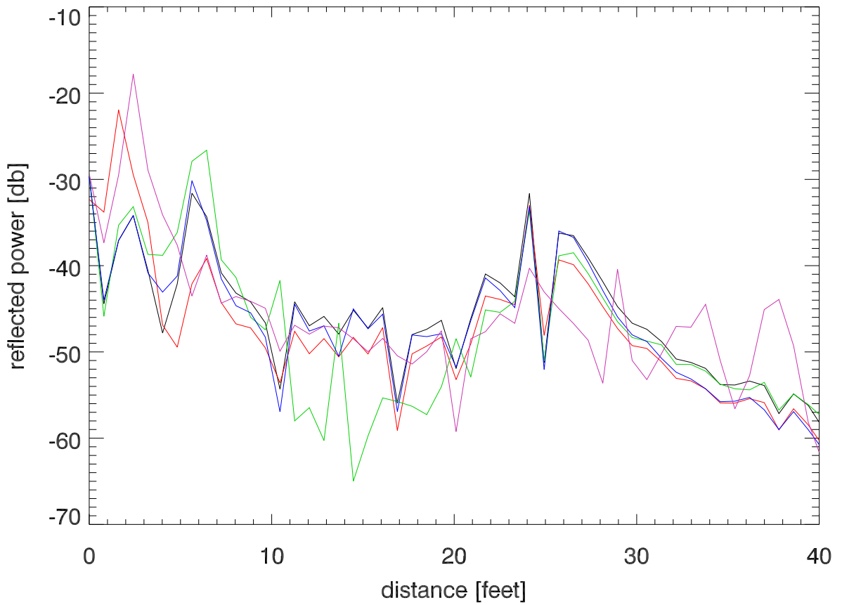
reflected power vs distance. vgrp=.817 (2380Mhz)
