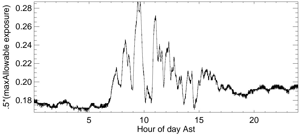
Rfmonitor data:090601
