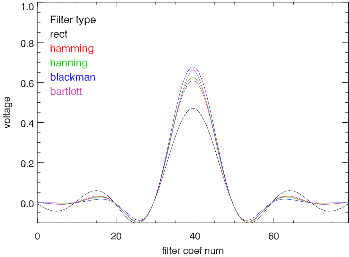
Time domain response Mock digFilt. dec= 10
