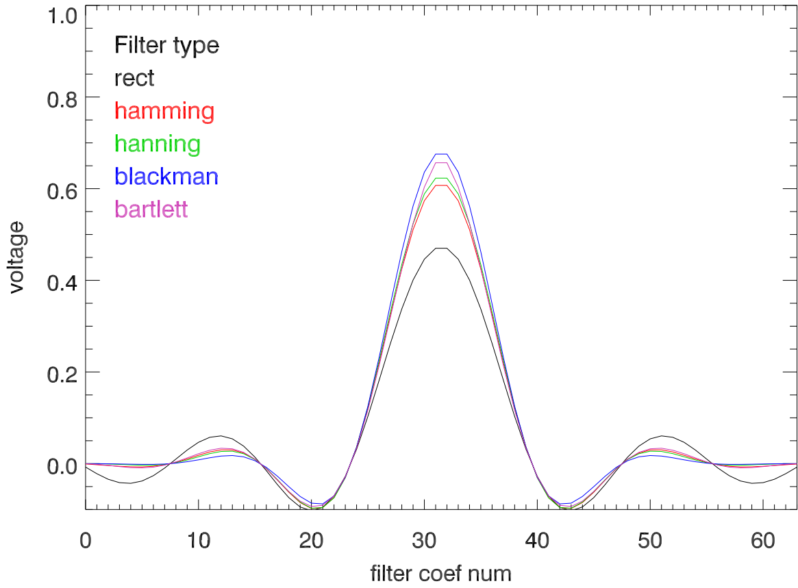
Time domain response Mock digFilt. dec= 8
