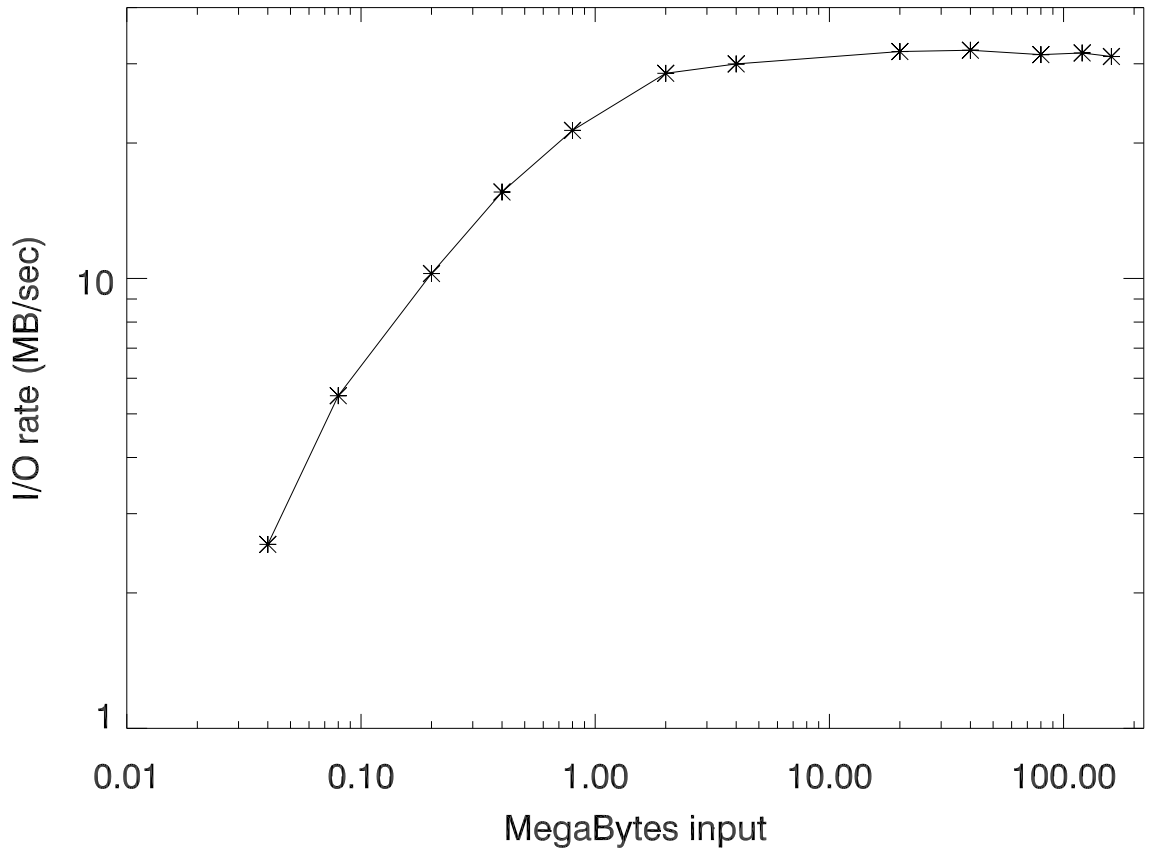
agilent 9104a transfer rate (gigabit ethernet)
