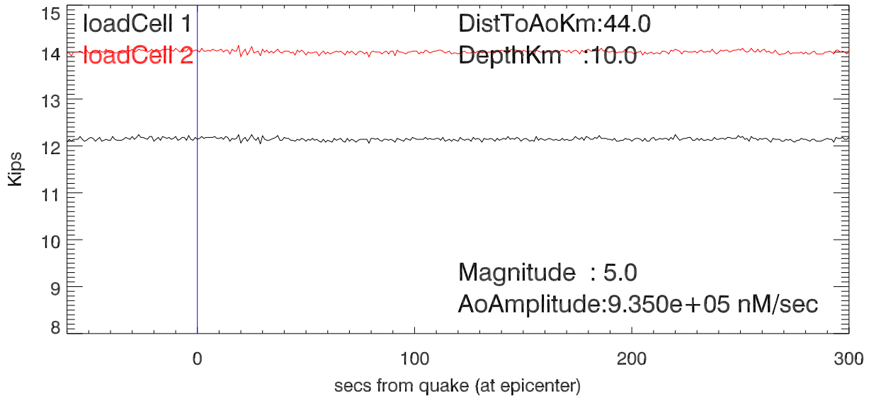
20200107 08:50:46(UTC) quake. tension in Td12
