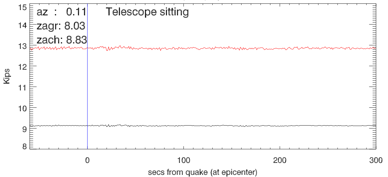
20200107 08:50:46(UTC) quake. tension in Td4
