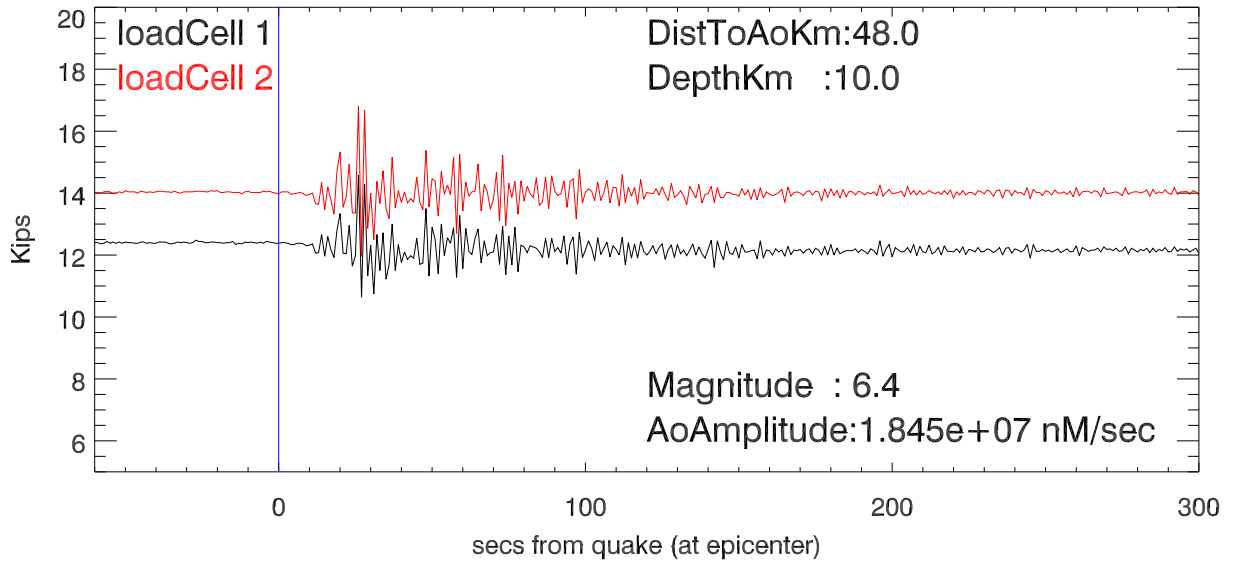
20200107 08:24:26(UTC) quake. tension in Td12
