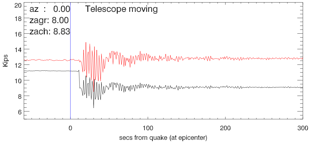
20200107 08:24:26(UTC) quake. tension in Td4
