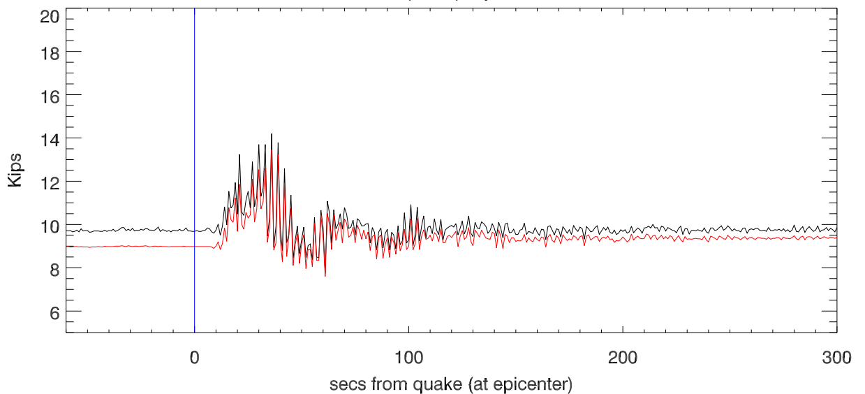
20200107 08:24:26(UTC) quake. tension in Td8
