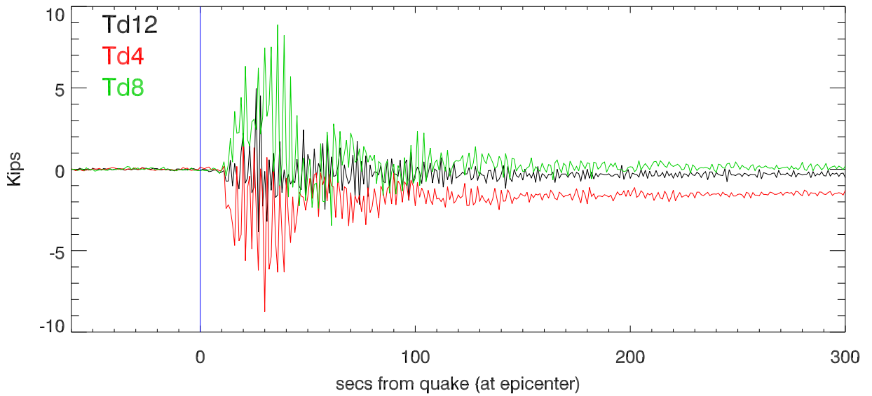
Kips change at each td corner vs time from epicenter
