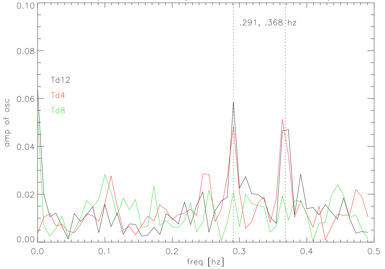
freq of oscillations (data from 40 to 150 secs)
