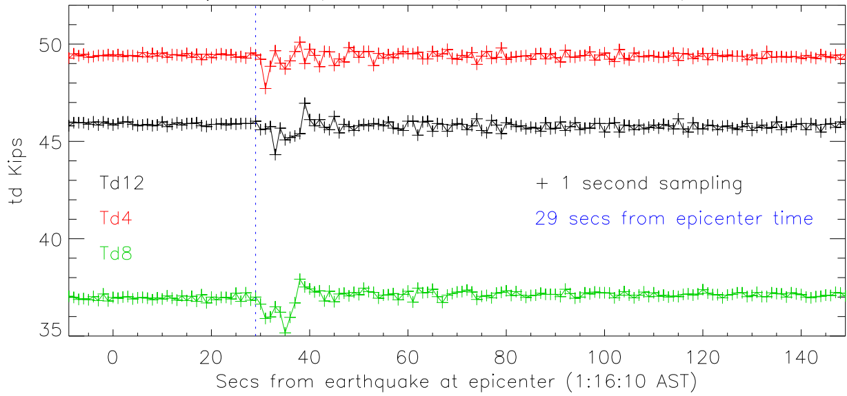
Change in kips vs time (remove median value, add offset)
