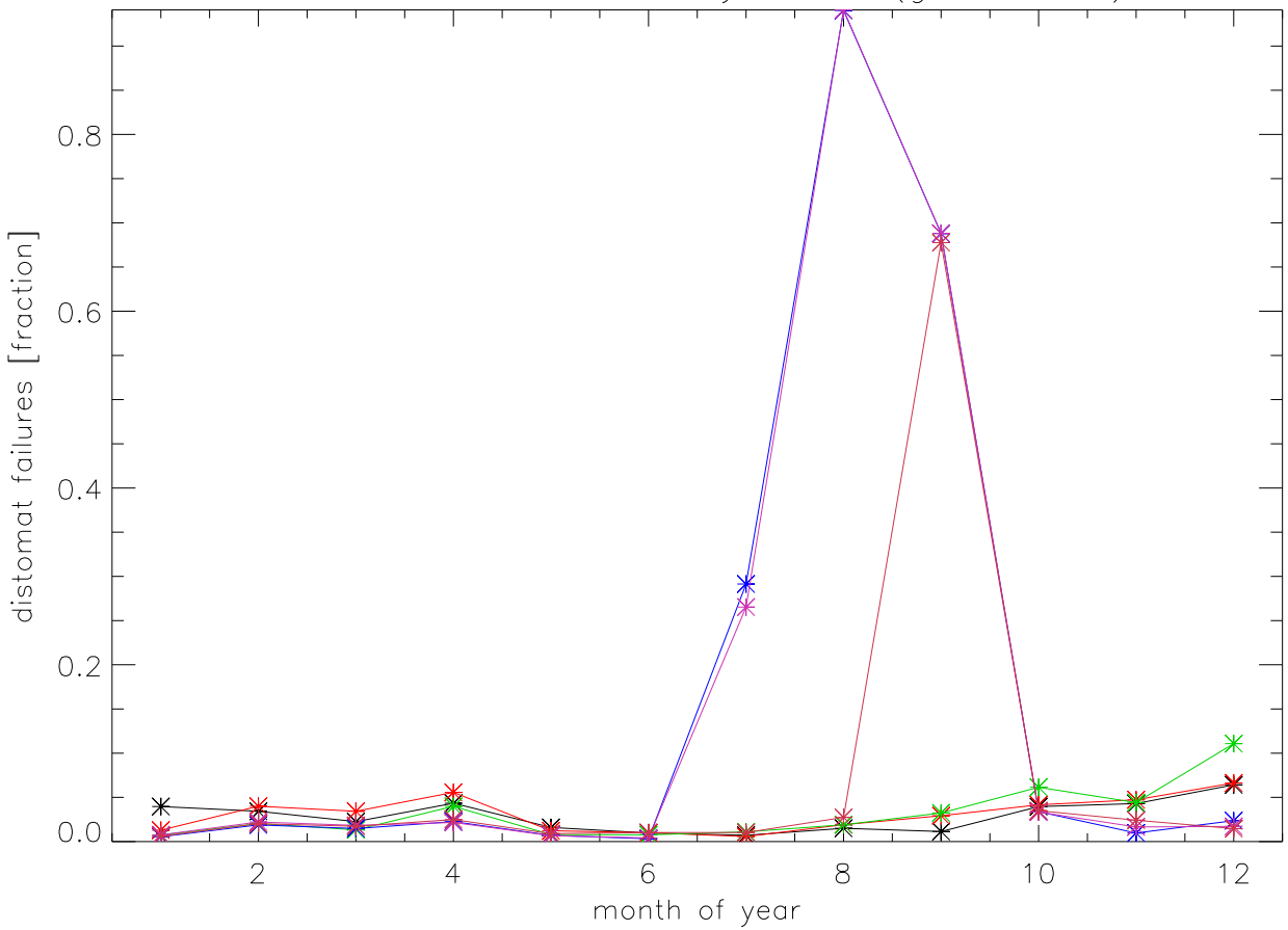
2007 distomat failures by month (gooddist=0)
