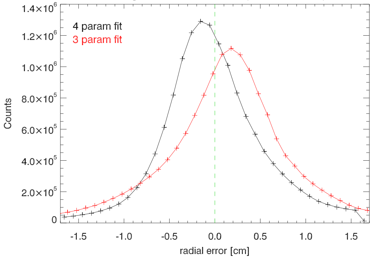
Histogram of radial errors (measured - fit)
