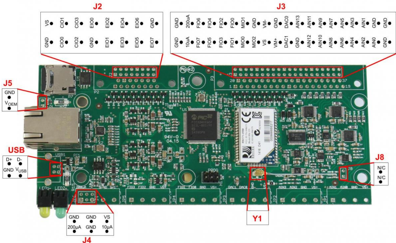
Image 22-3. T7-Pro-OEM Pinout
