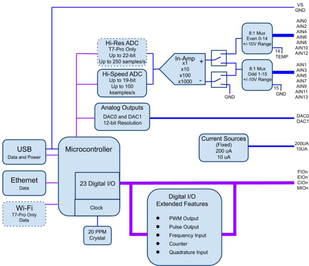
Figure 4.2-2. Block Diagram
